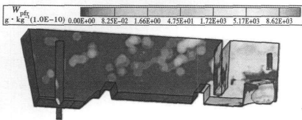
图 4 中间包夹杂物颗粒对耐火材料的冲蚀率分布 Fig. 4 Distribution of erosion-corrosion rate of refractory by inclusion particles in tundish
